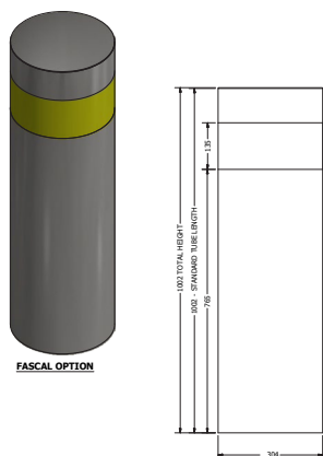
Sleeve + End Cap - Flat
