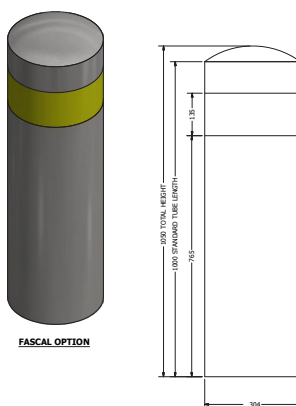
Sleeve + End Cap - Semi Dome
