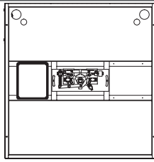
SECTION A-A SCALE 1 / 10
